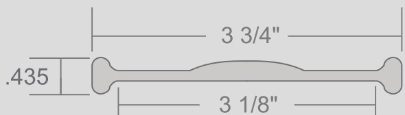
CROSS SECTION
